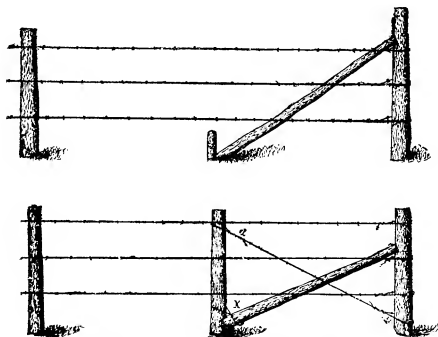
265. Bracing the end post.
